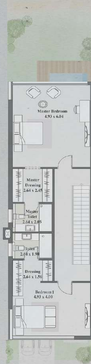
FIRST FLOOR
