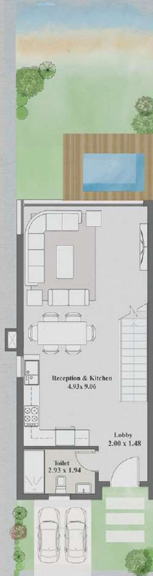
GROUND FLOOR
